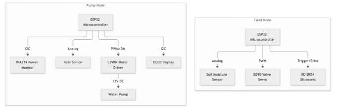
Fig. 2. Block diagram comparing the internal component architecture of the Field Nodes and the central Pump Node.
