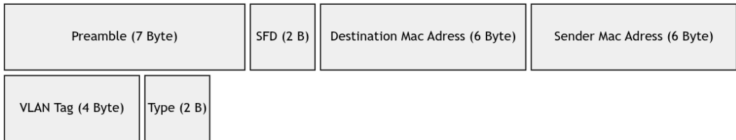
Figure 7: Ethernet Frame
