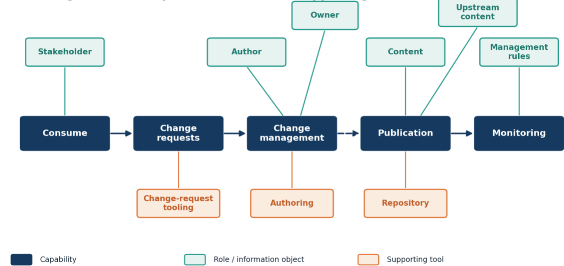
Figure A.1 — Semantic governance capabilities, the roles that carry them out, and the supporting application components.
