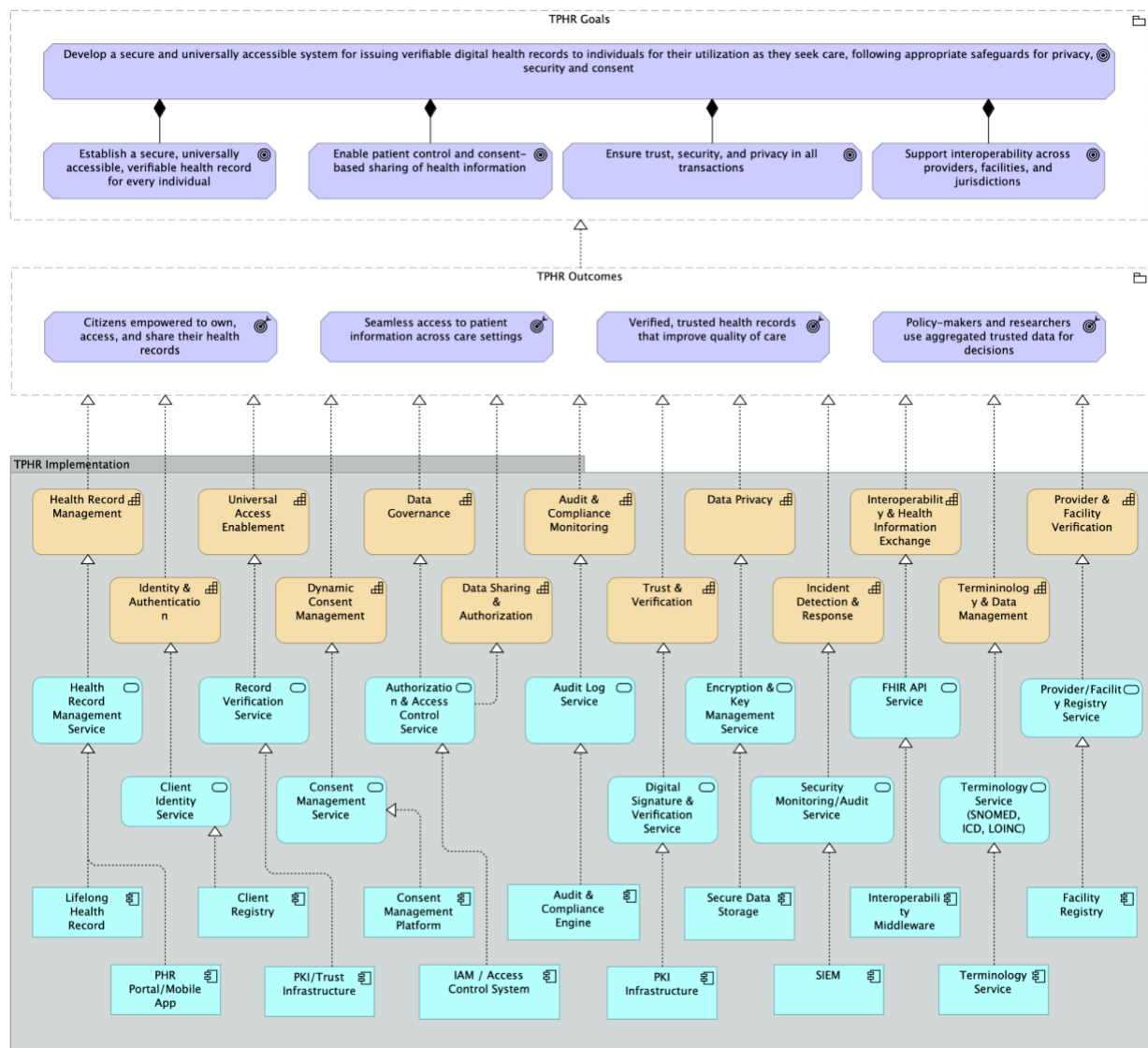
Figure 3.3: Simplified view of a single health goal (Establish Trusted Personal Health Records) — its sub-goals, the capabilities that enable them, the DPI-H components that support them, and the cross-cutting enablers
