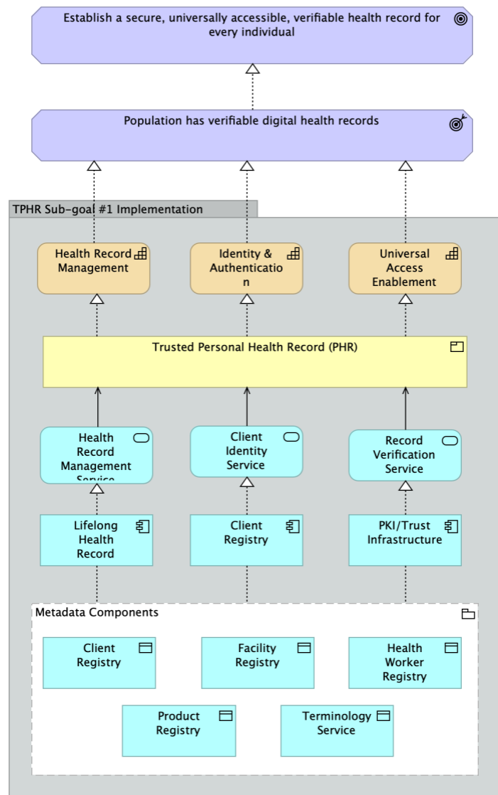
Figure 3.4: Layered view for one sub-goal relating to Establish Trusted Personal Health Records — from sub-goal and outcome, through capabilities and services, to metadata components
