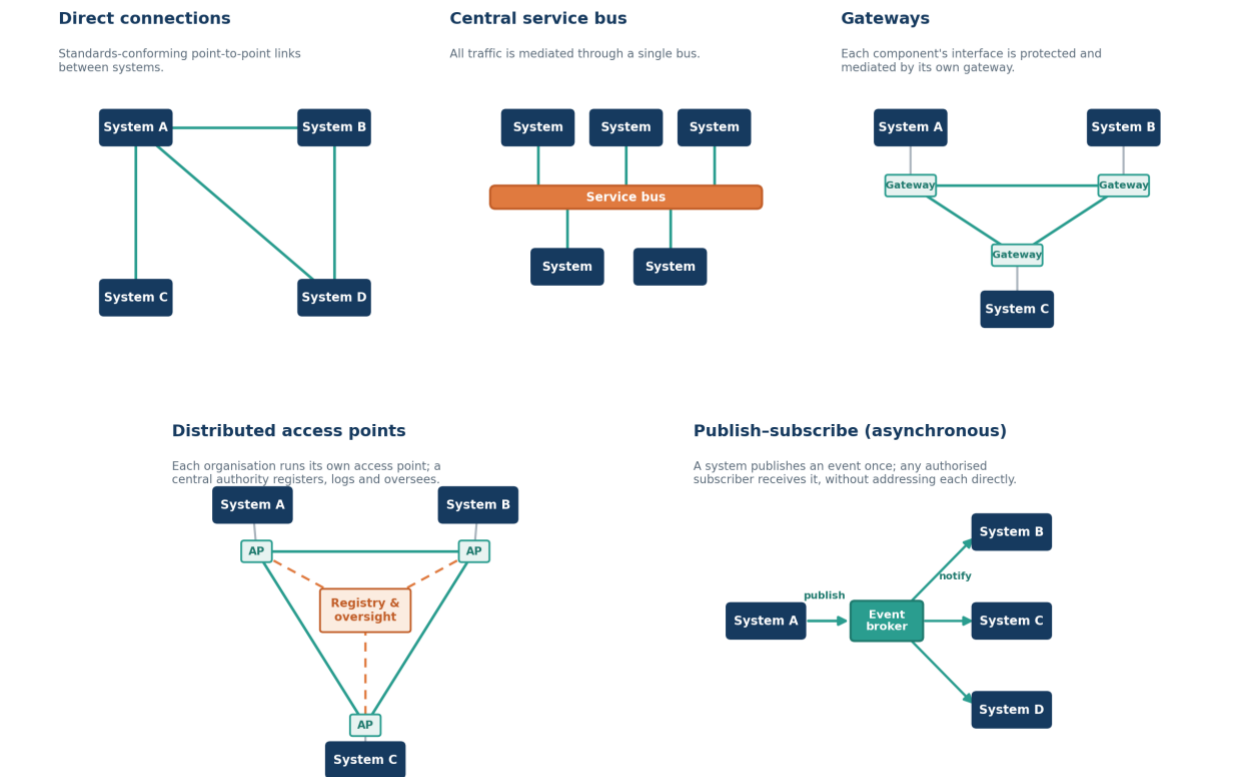
Figure 3.6 — Exchange patterns that can coexist within a single country. The same set of systems may be connected through any of these mechanisms, chosen according to context; the architecture does not prescribe one.
