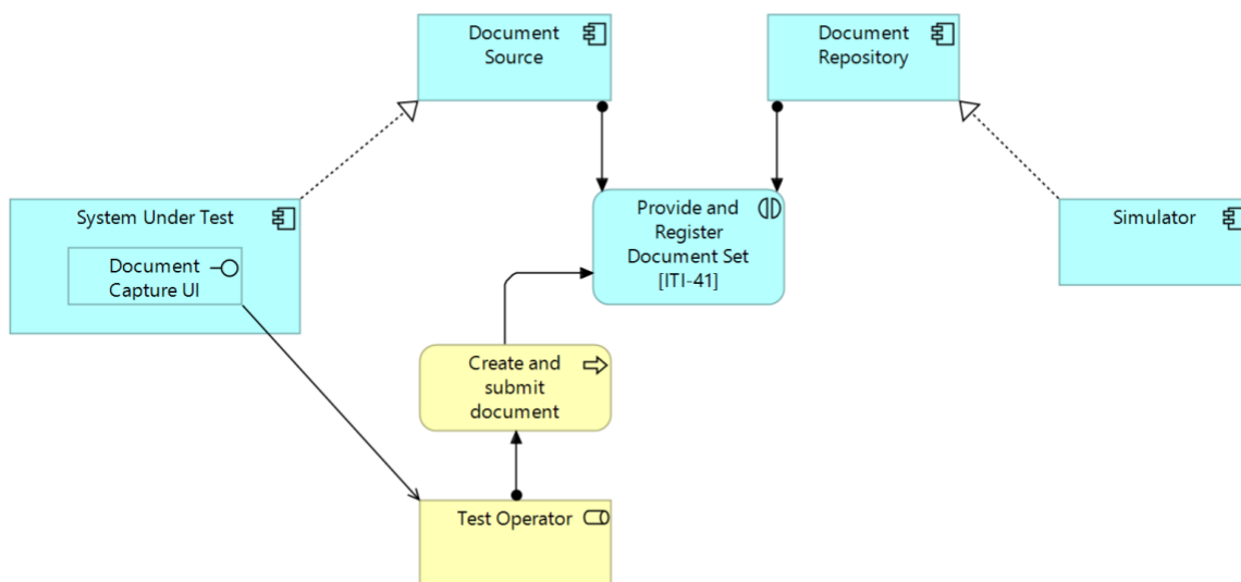
Figure 3.7.2. Conformance testing view. The System Under Test realises one actor role (here Document Source, the initiator) while a Simulator realises the opposite actor (Document Repository); both are assigned to the Provide and Register [ITI-41] interaction, so the test exercises one side at a time. The same system can also be driven through its UI: a Test Operator who creates and submits a document through the Document Capture UI triggers the same transaction — verifying the system end-to-end, as a user would, rather than by invoking the machine interface directly.
