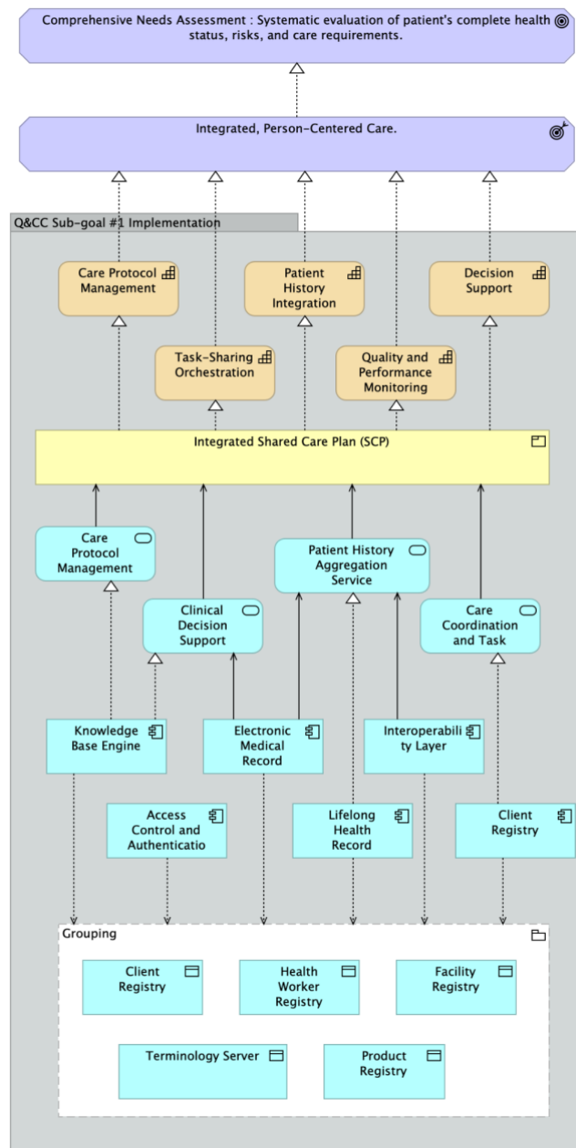
Figure 3.5: Layered view for one sub-goal relating to ensuring Quality and Continuity of Care — from sub-goal and outcome, through capabilities and services, to components and data
