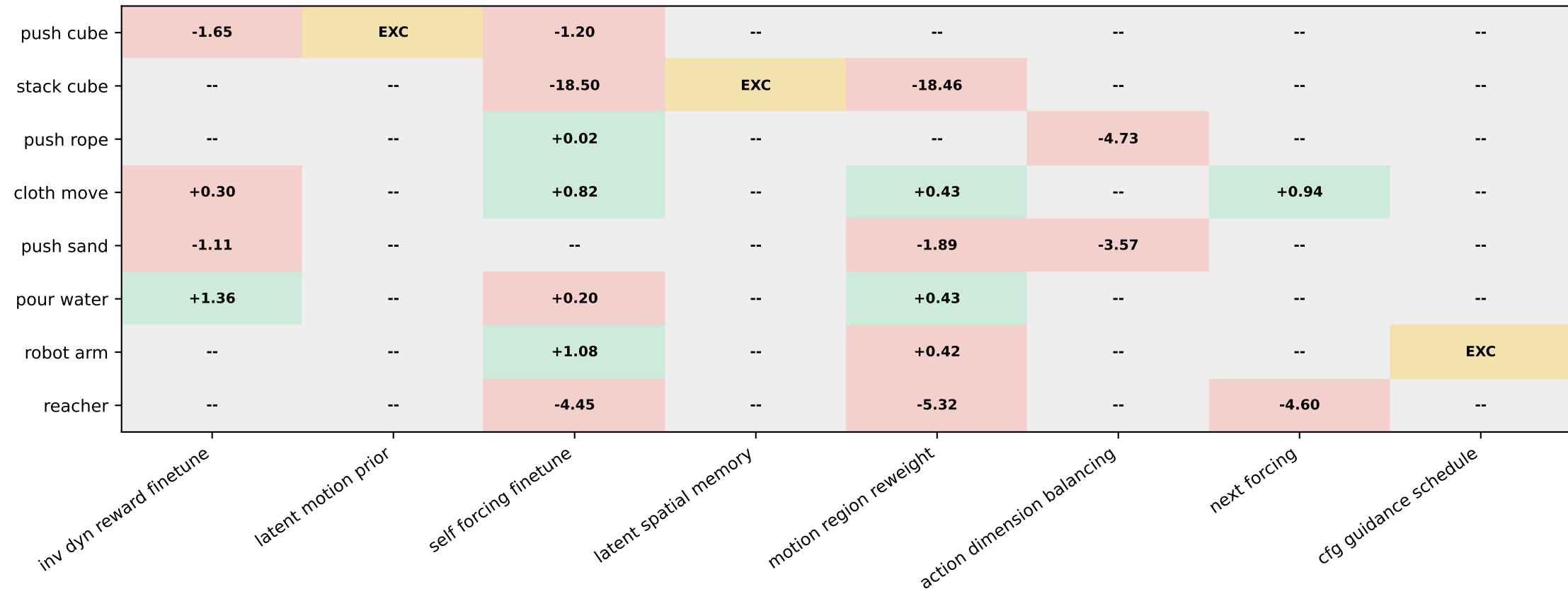
ACWM-Phys environment-by-primitive evidence
