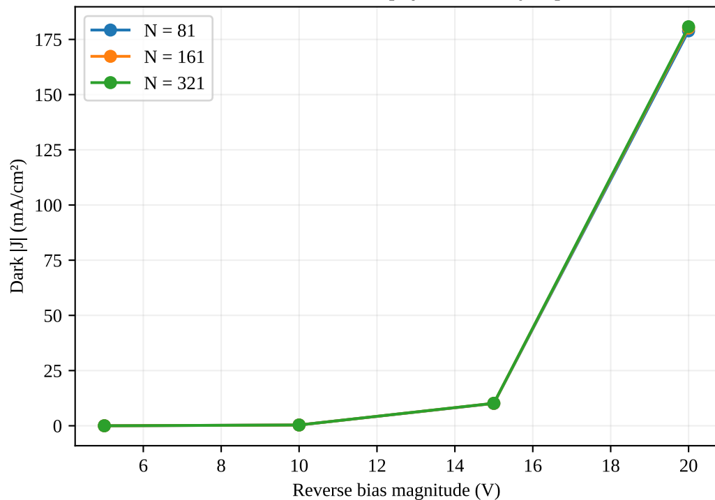
Mesh check: fixed physical 5 nm jumps
