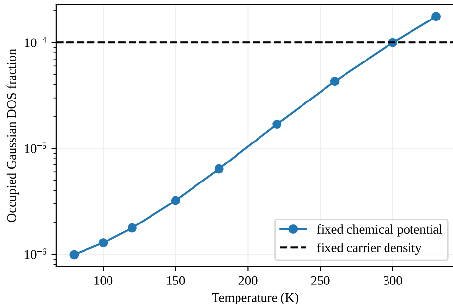
Equilibrium DOS illustration, \sigma=66.8 meV
