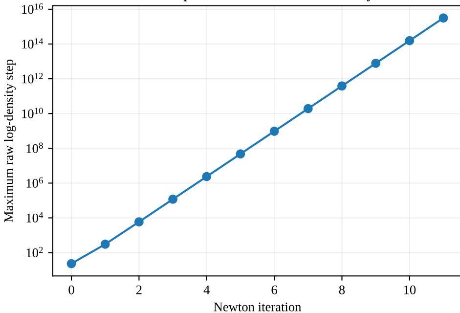
The depleted hole variable runs away
