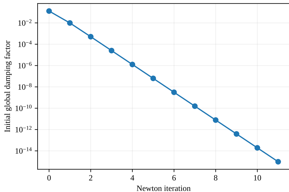
All variables become unable to advance
