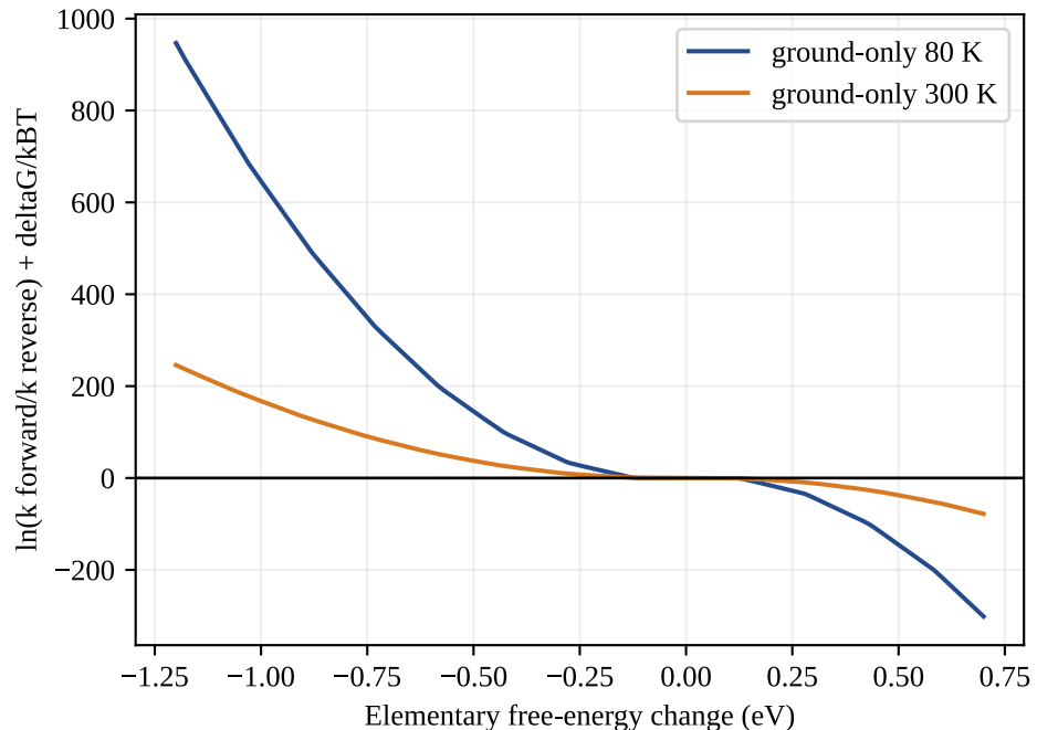
Exploratory H=10 micro-eV, total lambda=0.20 eV; exact thermal sidebands retain reverse processes
