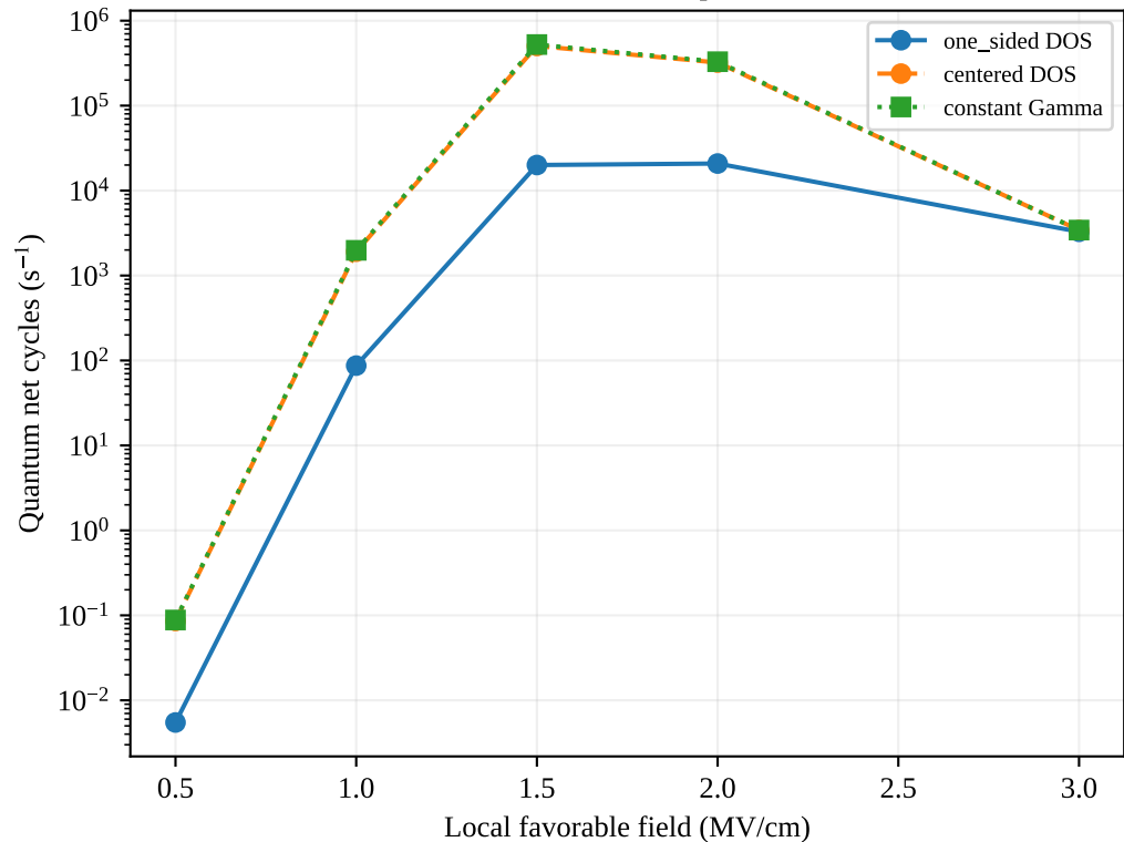
300 K; same reservoir H squared and width
