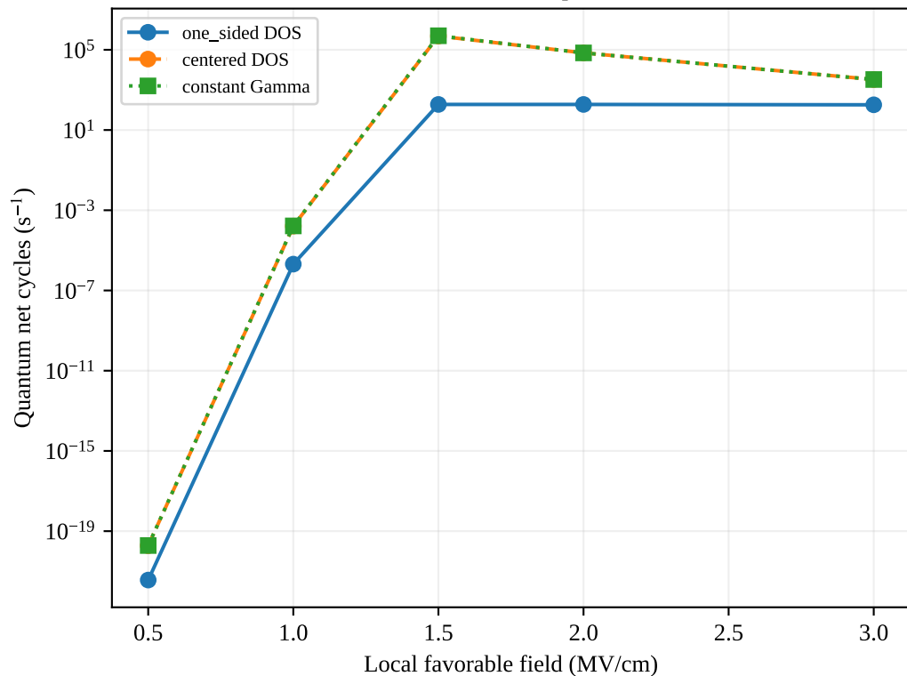
80 K; same reservoir H squared and width
