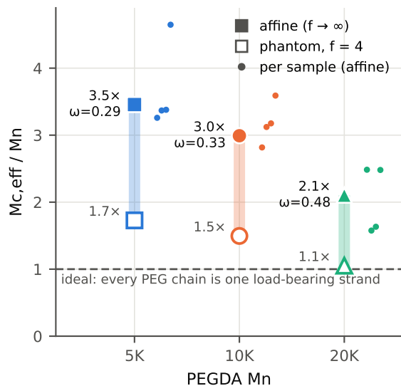
b Strand = 1.1–3.5 PEG chains in series
