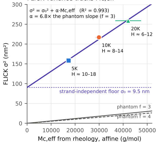
d FLICK variance tracks Mc, \text{eff}
