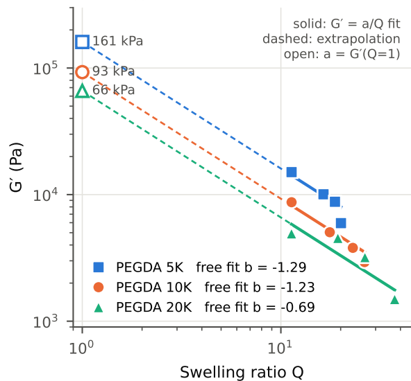
a Rheology: G' \propto 1/Q , extrapolated 10–30 \times to Q = 1
