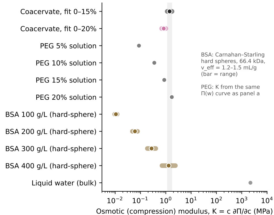
c How stiff is \sim 1 MPa?
