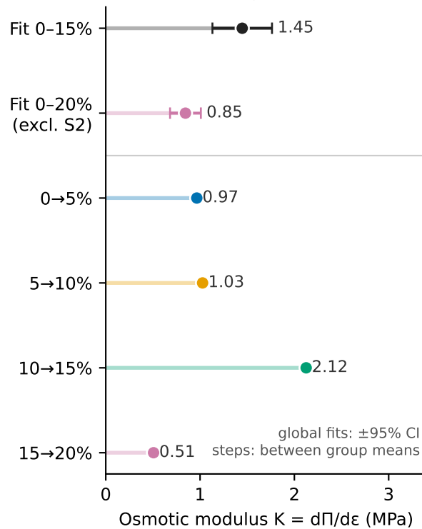
b Modulus, global and local
