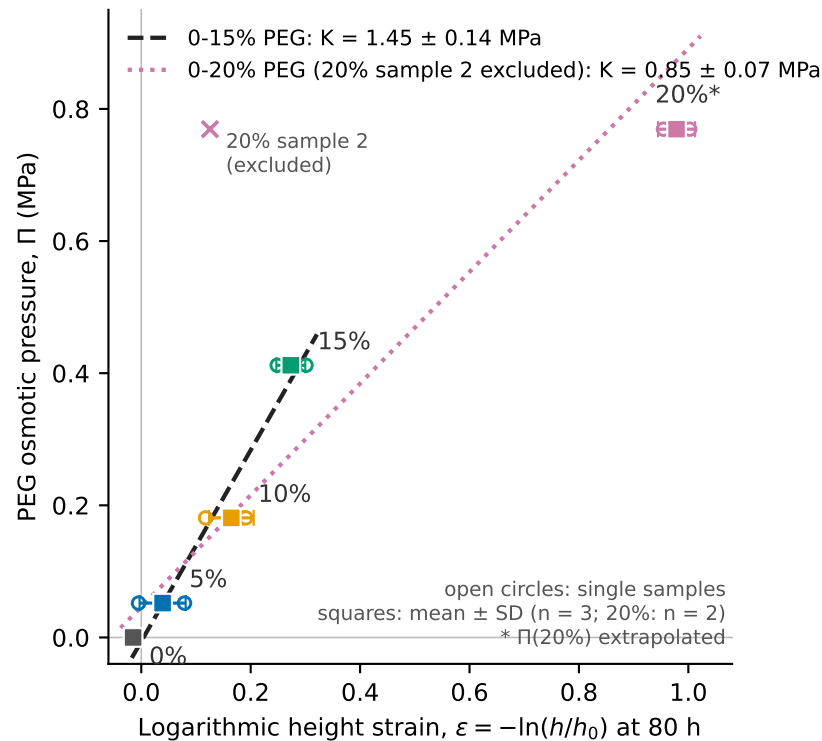
a Equation of state from osmotic compression
