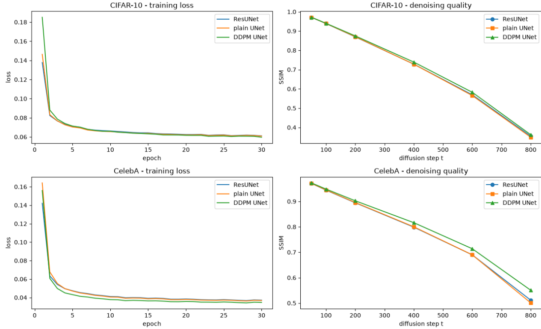
Figure 3.4: Training loss (left) and denoising accuracy against noise level (right) for CIFAR-10 (top) and CelebA (bottom).
