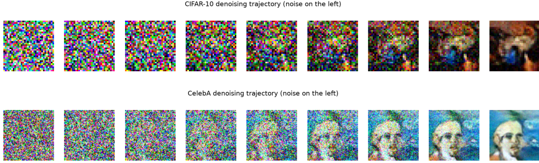
Figure 3.3: Reverse trajectories of the proposed network on CIFAR-10 (top) and CelebA (bottom), with pure noise on the left and the final sample on the right.
