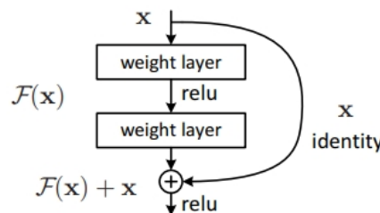
Figure 2.1: Residual Learning: a building block [2]
