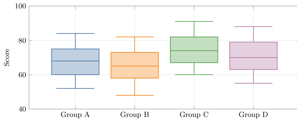
Figure 6: Box plot showing score distributions across groups.
