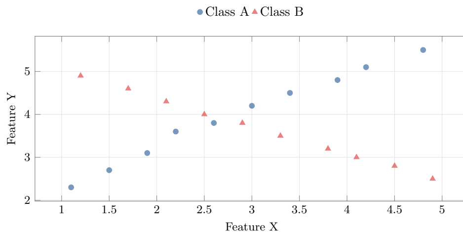
Figure 4: Scatter plot showing two synthetic feature groups.
