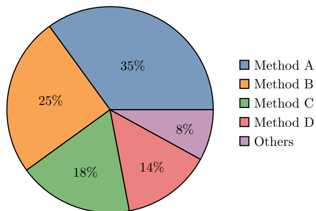
Figure 5: Pie chart showing the proportion of different methods.
