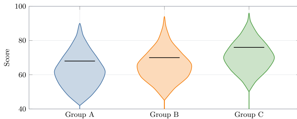
Figure 8: Violin plot showing synthetic score distributions.
