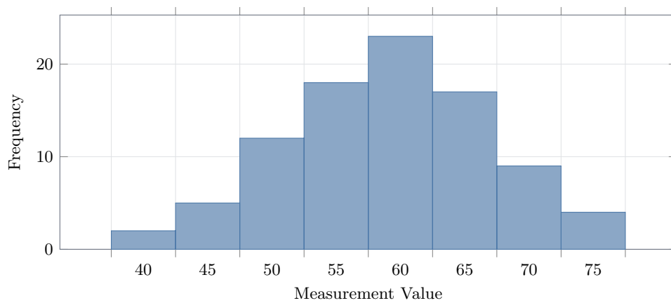
Figure 2: Histogram showing the distribution of measurement values.
