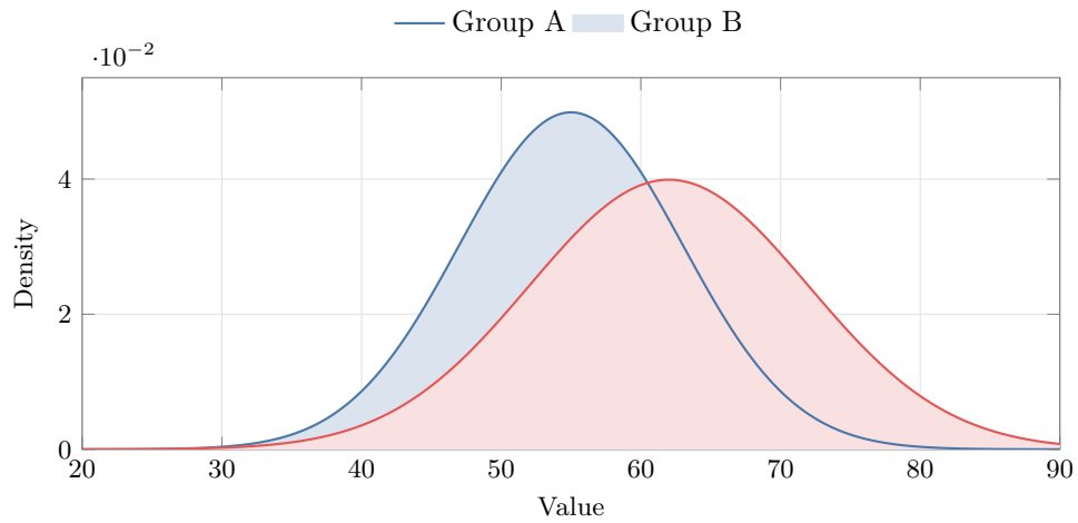
Figure 7: Density plot comparing two synthetic distributions.
