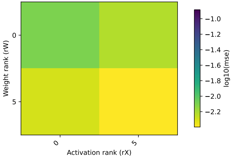
Final Hidden State \log_{10}(\text{mse}) Heatmaps
