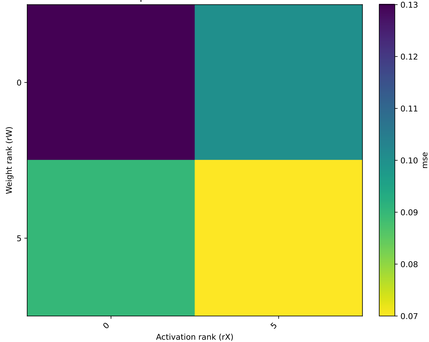
nvfp4 Final Hidden State mse
