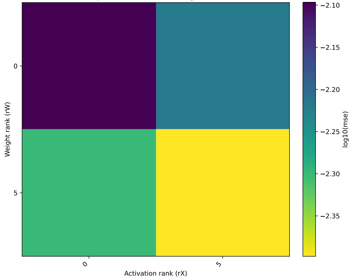
nvfp8 Final Hidden State \log_{10}(\text{mse})
