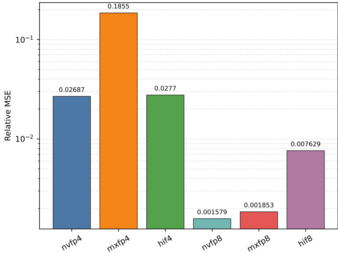
Quantization Format Comparison on Final Hidden Representations Final Hidden State MSE (log scale) Relative MSE (log scale)
