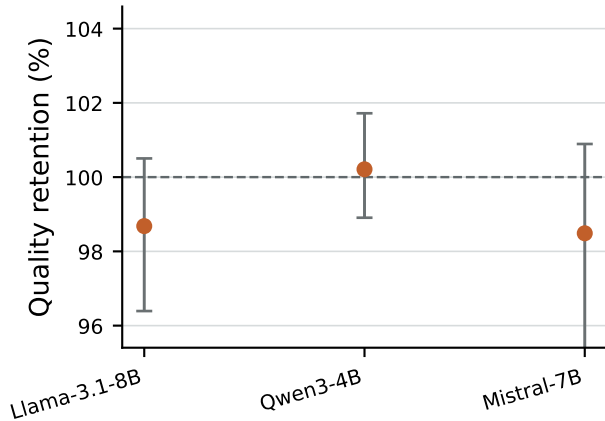
(b) Model transfer
