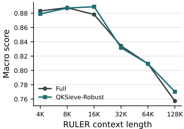
(a) Length generalization
