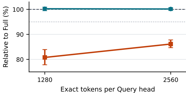
(a) Causal-PPL retention
