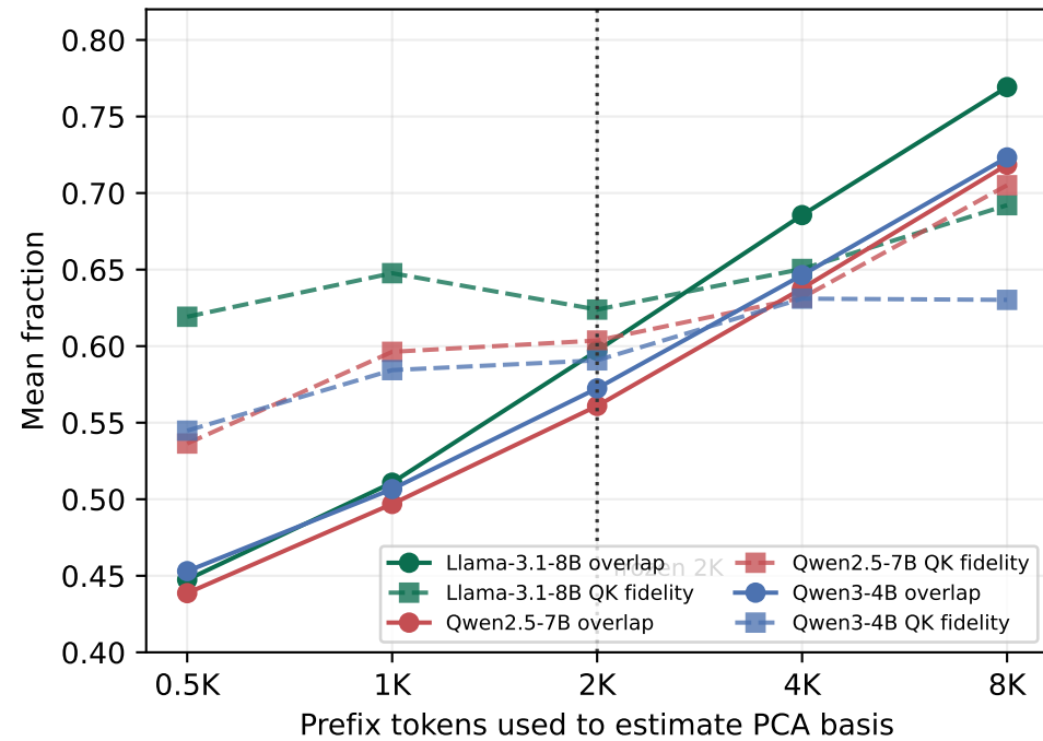
(a) Prefix basis drift
