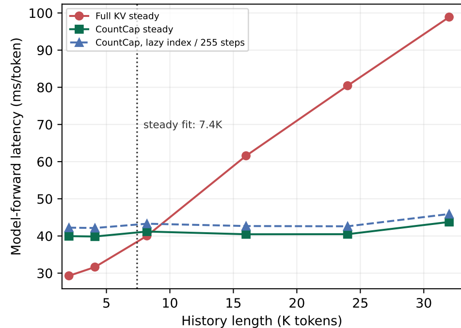
(c) Steady and amortized cost
