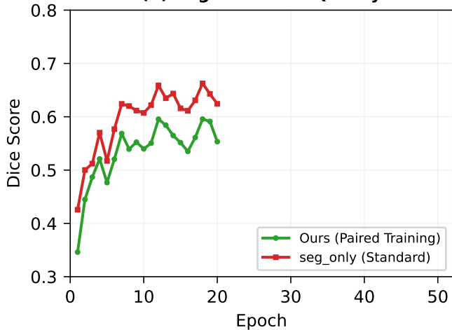
(b) Segmentation Quality
