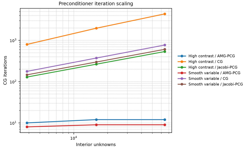
Figure 5. Iteration scaling for the solver comparison. AMG-PCG keeps iteration counts nearly flat over the tested grid sizes for these cases.
