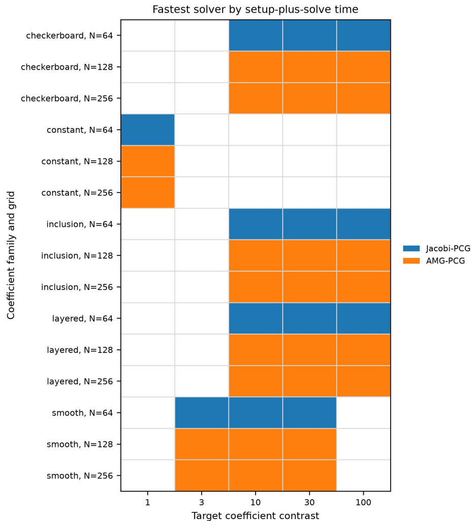
Figure 3. Fastest converged solver by setup-plus-solve time over the coefficient-family grid.
