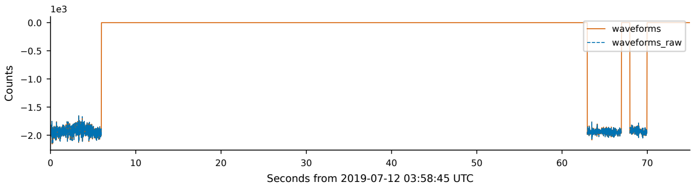
c Added horizontal channels · CI.WNM
