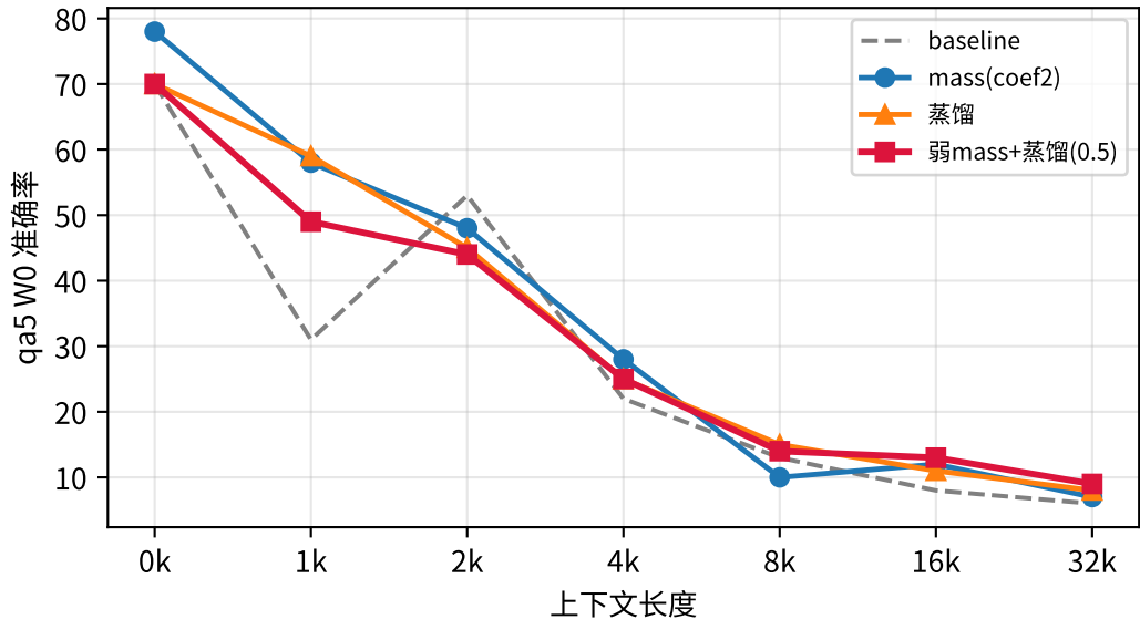
四类杠杆 W0 readout (BABILong qa5)
