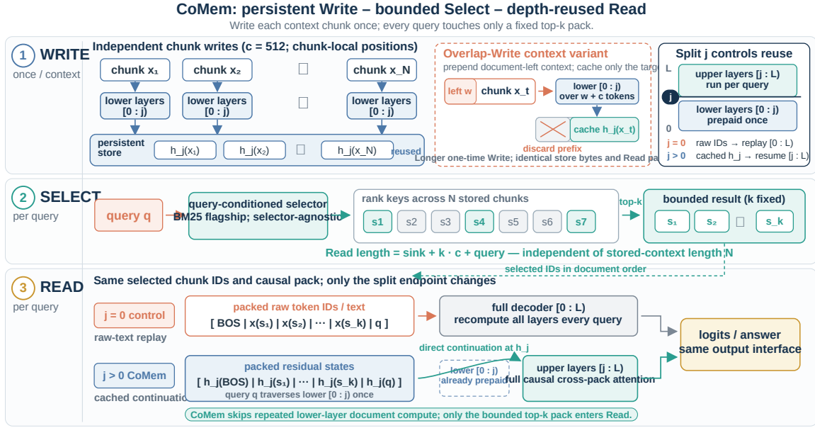
Figure 1: CoMem turns transformer depth into a cross-query reuse axis. WRITE pre-pays layers [0:j] once per document chunk, SELECT retrieves a bounded working set, and READ resumes [j:L] with the query present. The matched j=0 endpoint uses the same selected chunks, order, sink, mask, and adapter while replaying all layers, thereby isolating the incremental depth effect. Overlap-Write supplies a small amount of left document context without enlarging the stored object or Read pack.
