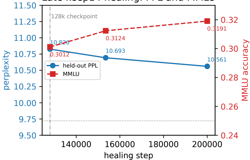
Late keep14 healing: PPL and MMLU
