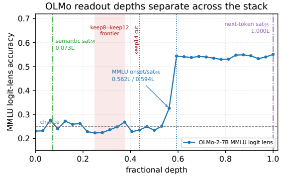
Figure 6: Probe-dependent readout depths on OLMo-2-7B . The shaded band marks prefix cuts used by the available behavioral points. Thresholds use different readouts and are descriptive; they are neither directly comparable causal boundaries nor locations of stored knowledge.
