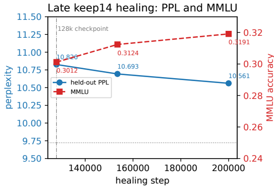
Figure 1: Late keep14 healing continues on both axes, but the remaining capability gap is large. From 128k to 200k, PPL improves from 10.826 to 10.561 and MMLU from .3012 to .3191; the intact base remains at .6053 MMLU. The figure supports slow late recovery, not a claim that MMLU is numerically constant.
