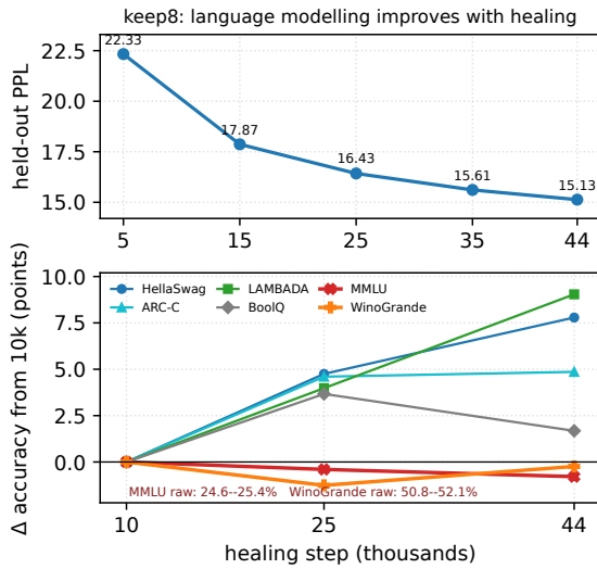
Figure 4: The shallow keep8 arm improves in likelihood and ordinary tasks through 44k. The retained 44k and 121k aggregate checkpoints both remain near MMLU chance; the comparison is descriptive because the available run lacks seed replication.
