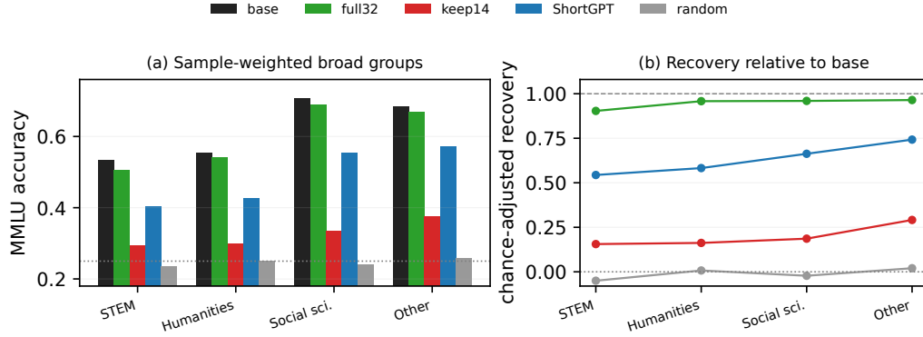
Figure 3: MMLU recovery is heterogeneous across broad domains. Accuracy is sample weighted over the standard four MMLU groups. Recovery is chance adjusted, (a - 0.25)/(a_{\text{base}} - 0.25) . Full32 remains close to the base in every group; ShortGPT consistently exceeds keep14, but neither half-depth arm closes the intact-model gap.
