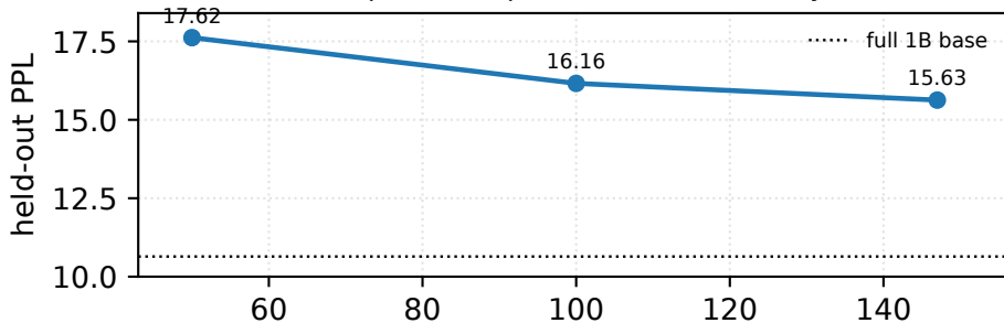
OLMo-2-1B keep7: PPL improves while MMLU stays at chance
