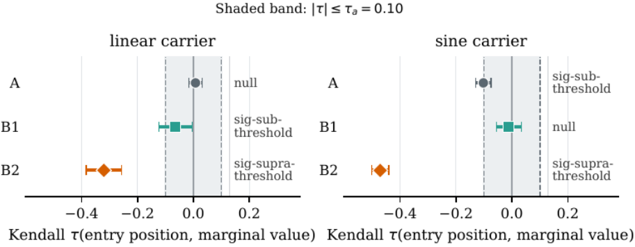
Figure 2: Frozen six-cell construction sensitivity (16 seeds per cell), extracted from the supplied PDF. Points are mean per-seed Kendall \tau ; bars are 95% Student- t intervals; the shaded band is |\tau| \leq \tau_a = 0.10 . Exact values appear in Table 2.
