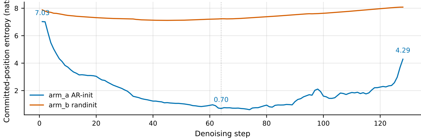
Committed-position entropy over denoising, \tau = 0.7 (descriptive; control is near-untrained)
