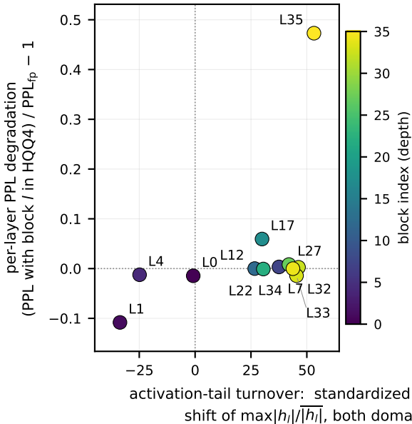
Qwen3-4B — 12 of 36 blocks probed \rho(\text{turnover}, \text{degrad}) = +0.559
