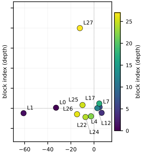
Qwen3-1.7B — 11 of 28 blocks probed \rho(\text{turnover}, \text{degrad}) = +0.118
