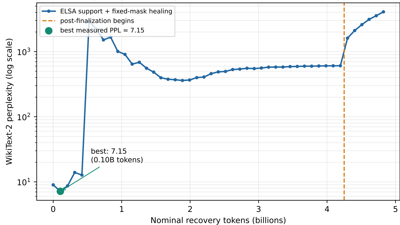
Long-budget recovery with a fixed ELSA-derived 2:4 support
