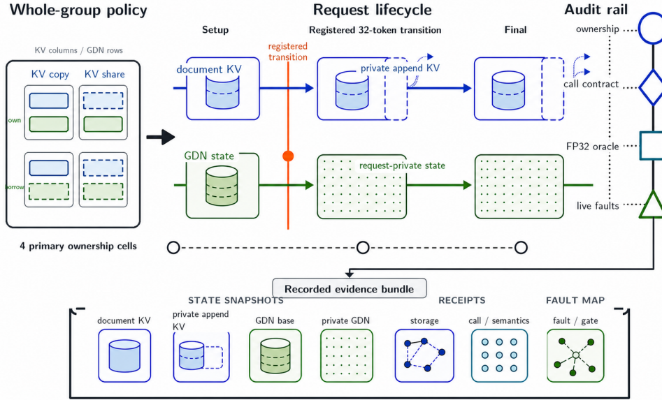
Figure 2: FORKAUDIT ownership factorial. Four KV-by-GDN setup cells share immutable document state, keep append tails private, and rebind borrowed recurrent state at the registered transition. The audit rail records lifecycle, storage, call/semantic, and fault-to-gate receipts. This schematic details the validation component; it is not experimental evidence.
