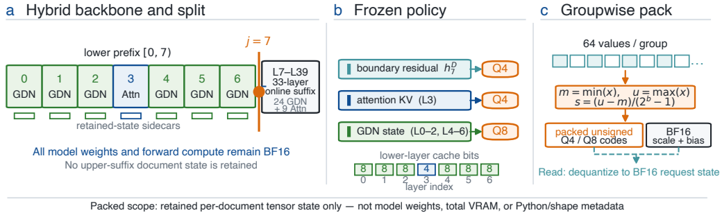
Figure 2: Quantization scope and frozen Q4/Q4/Q8 policy. (a) At split j = 7 , the retained entry contains the boundary residual and state sidecars from lower layers L0–L6; model weights and forward computation remain BF16, and L7–L39 document state is reconstructed during Read rather than retained. (b) The frozen state-type point packs h_j^D and L3 attention KV at Q4, and the L0–L2/L4–L6 GDN convolution/recurrent state at Q8. (c) Each 64-value group stores packed unsigned codes plus BF16 scale and bias, and is dequantized to BF16 request state on Read. Q16 denotes the unpacked BF16 reference. The scope is retained tensor payload, not model weights or total VRAM.
