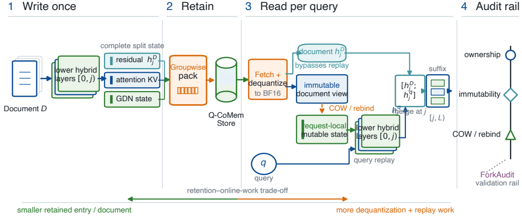
Figure 1: Q-COMEM protocol geometry. Write runs a document once to split depth j and packs the complete retained state: boundary residual, lower full-attention KV, and lower GDN convolution/recurrent state. Read dequantizes that entry, exposes immutable document tensors, creates request-local mutable state through COW/rebinding, and replays the query through [0, j] . The document and query residuals merge only at j before suffix execution and decoding. The narrow FORKAUDIT rail validates the ownership boundary; it is not an additional execution stage.
