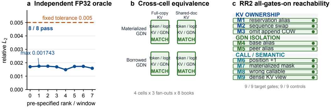
Figure 3: Primary validation. Left: all selected attention rows beat the pre-fixed tolerance. Center: four ownership cells match on registered observables. Right: a separate RR2 all-gates-on reference reaches every target gate with passing controls. Together these panels connect selected numerical agreement, cross-cell invariance, and targeted violation localization.
