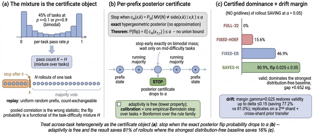
Figure 1: Conceptual overview with artifact-checked quantitative labels. (a) Treat across-task heterogeneity as the certificate object: per-task pass rates are strongly bimodal, so the flip probability is a functional of the difficulty mixture H , not of a pooled correlation. (b) BAYES-H stops when the exact posterior flip probability c_H(x, k) drops to \alpha ; by the tower property adaptivity is free (no union bound), and calibration is one empirical-Bernstein step over tasks. (c) At \alpha = 0.05 BAYES-H has an 80.9% replay rollout-count reduction (realized flip 0.025), dominating the strongest distribution-free baseline (FIXED-HOEF, 15.6%) and the strongest mixture-aware fixed budget (FIXED-EB, 46.9%); a certificate margin controls flip only in stated synthetic drift mechanisms, and all results replicate on a disjoint second shard. Panel (c)’s displayed numbers are rounded reproductions of the named replay artifacts, not measurements generated by the figure. The flip and count quantities are replay artifacts, not online correctness or operational-cost measurements (REPRO_README.md).
