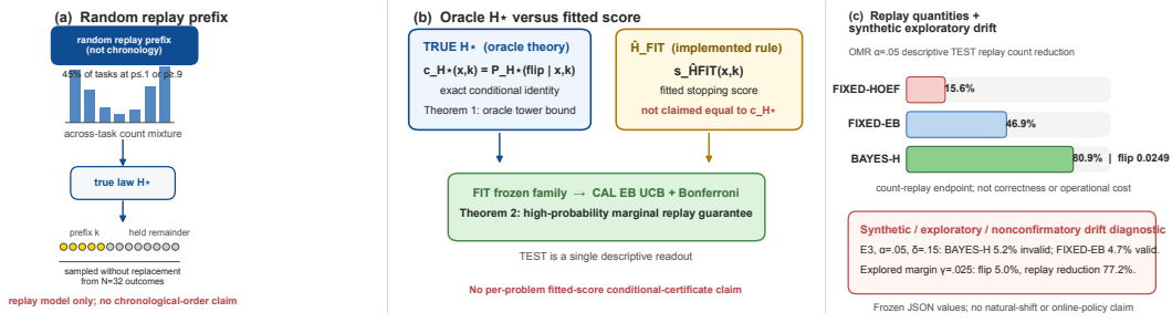
Figure 1: Code-native overview; frozen-JSON labels. (a) A random replay prefix is not chronological. (b, left) only the true count law H_* gives the exact conditional identity for c_{H_*} and the oracle tower theorem. (b, right) BAYES-H uses the distinct fitted score s_{\hat{H}_{\text{FIT}}} ; its operational claim is the FIT-frozen, Bonferroni CAL-EB UCB screen of Theorem 2, not an exact per-problem conditional certificate. (c) The shown replay quantities are parsed from hash-pinned frozen JSON; the drift/margin note is synthetic, exploratory, and nonconfirmatory. The figure supplies no ordered-online, correctness, or operational-cost measurement.
