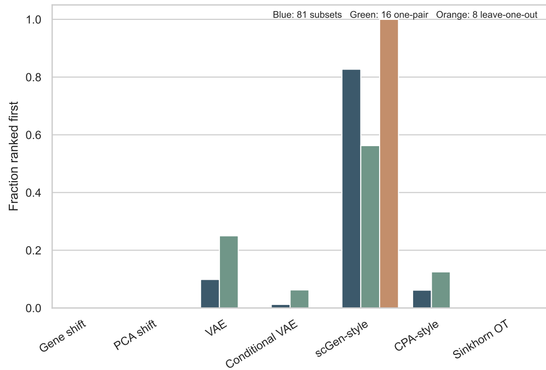
First-place frequency under animal removal
