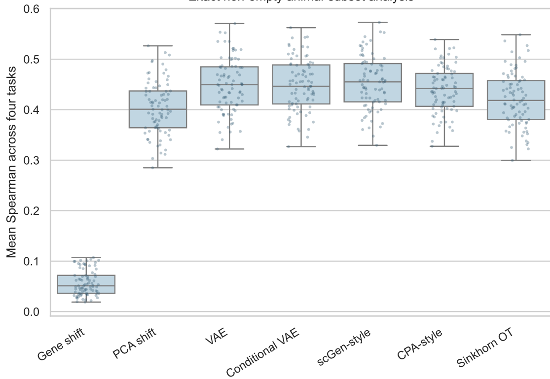
Exact non-empty animal-subset analysis
