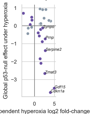
C Global p53 loss reverses 16/28 evaluable signature genes
