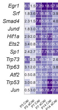
C Global p53 loss reverses 16/28 evaluable signature genes
