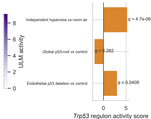
C Global p53 loss reverses 16/28 evaluable signature genes
