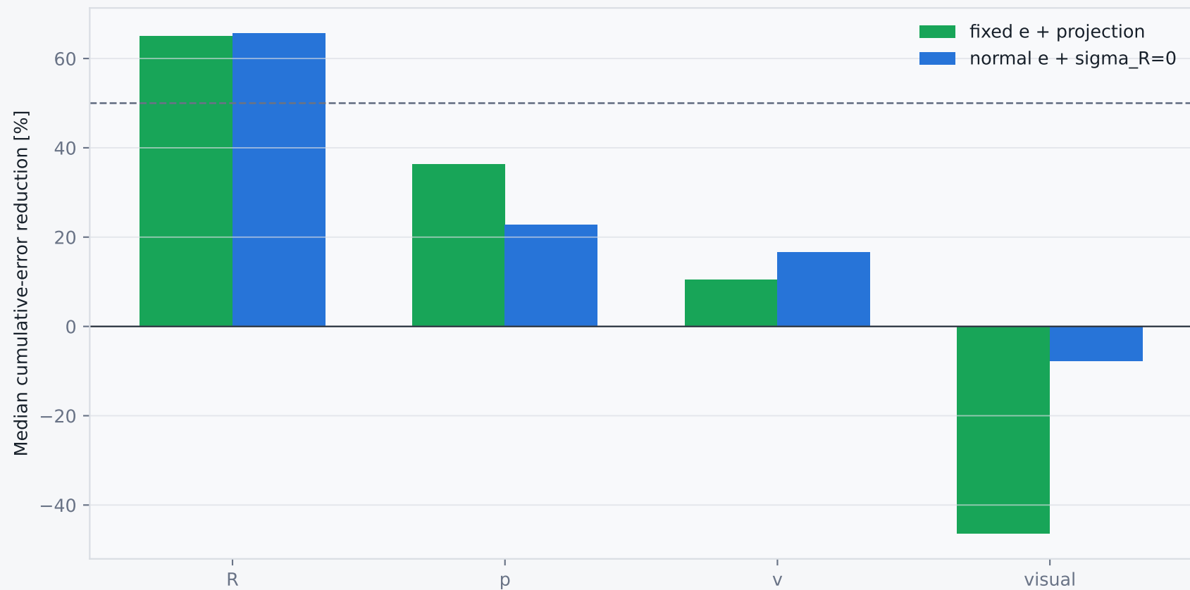
Causal interventions relative to baseline
