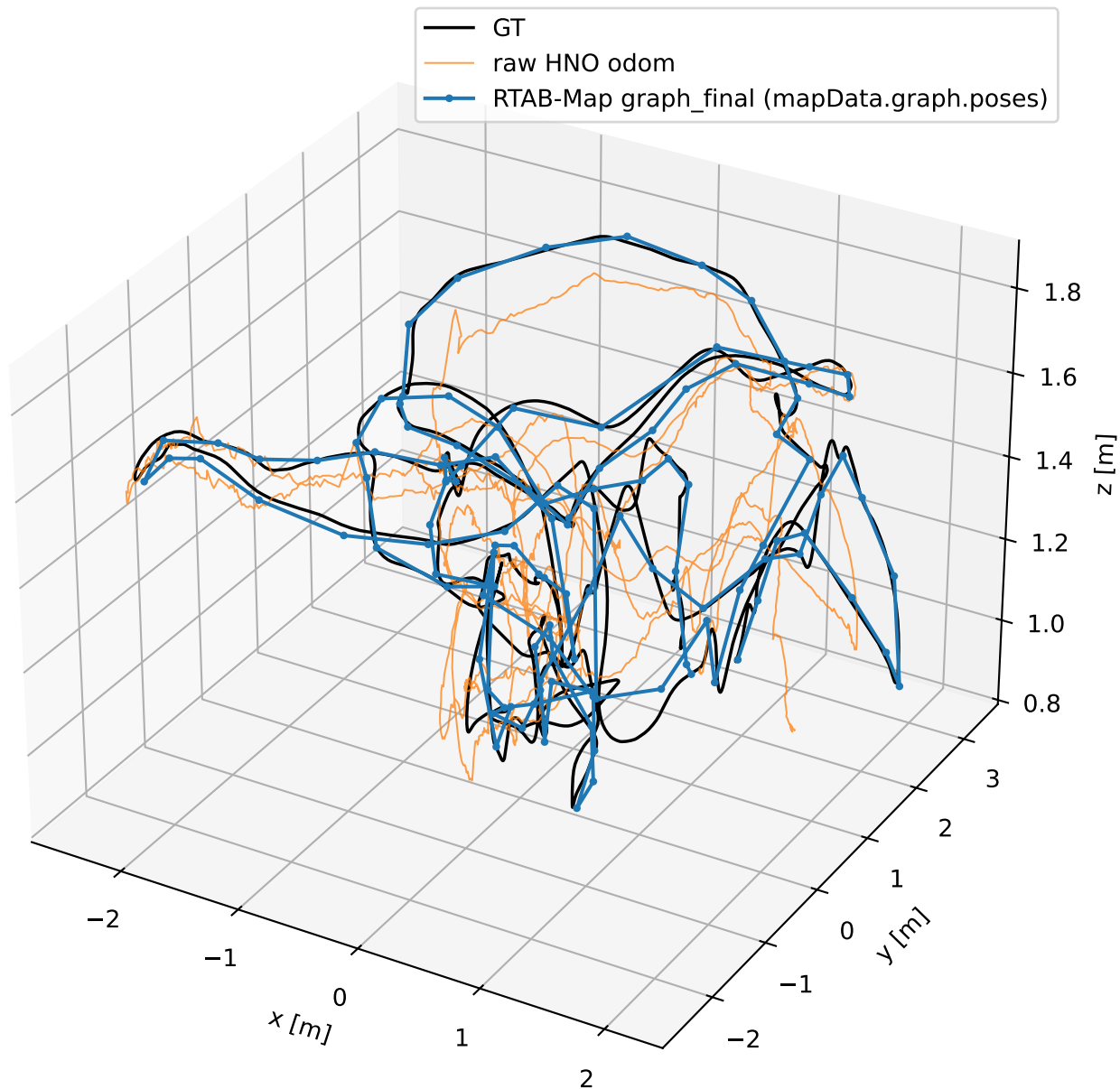
3D: GT vs raw vs graph_final, Sim(3) aligned
