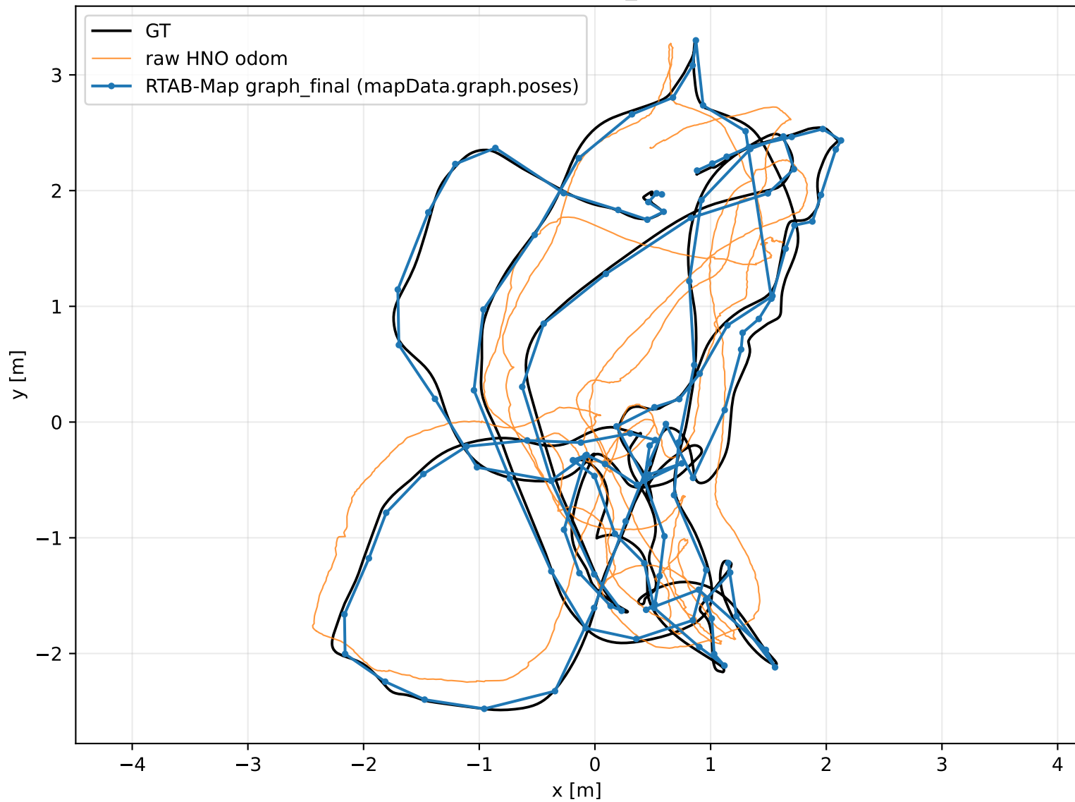
GT vs raw vs RTAB-Map graph_final, Sim(3) aligned
