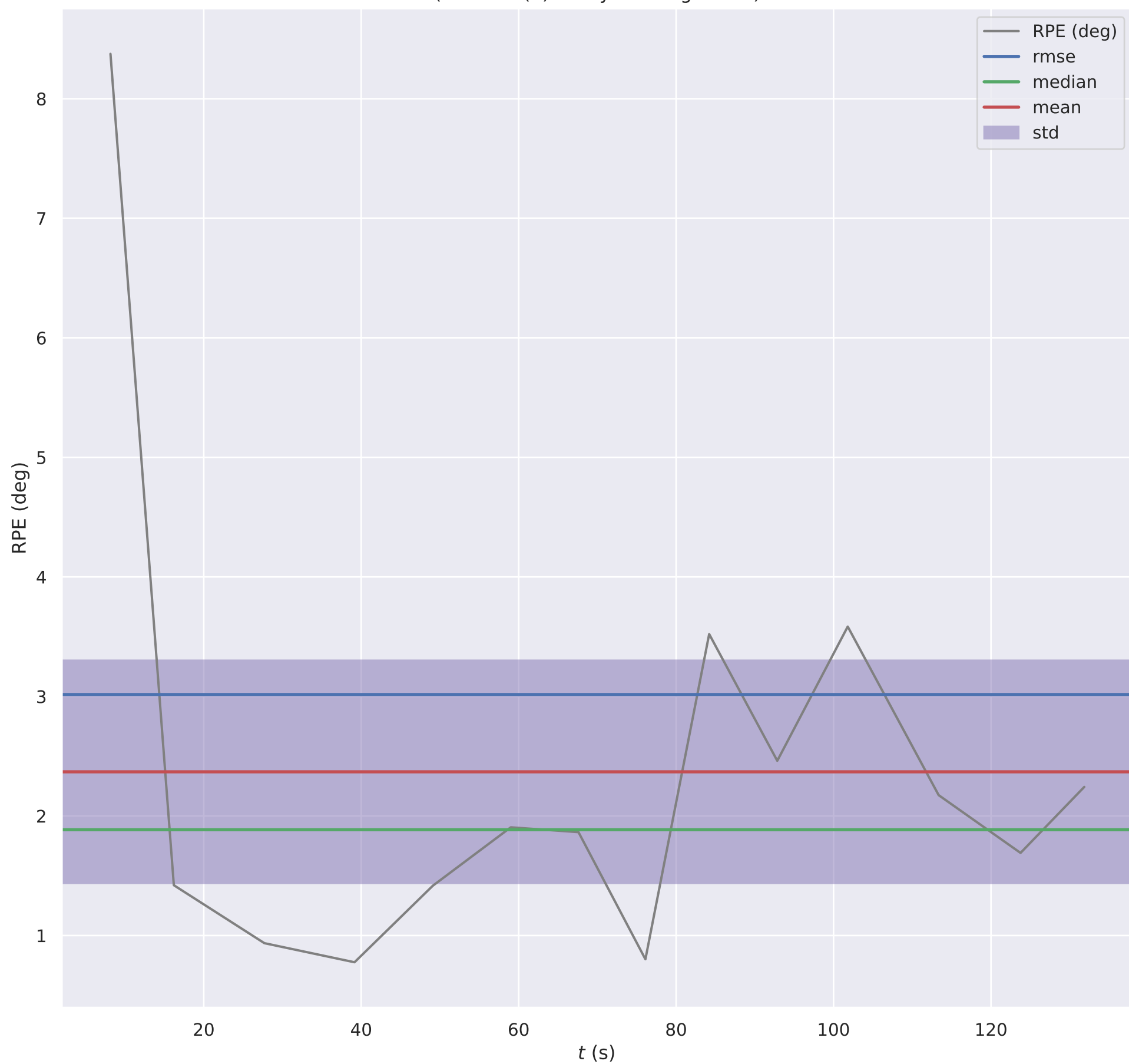
RPE w.r.t. rotation angle in degrees (deg) for \delta = 20 (frames) using consecutive pairs (with Sim(3) Umeyama alignment)
