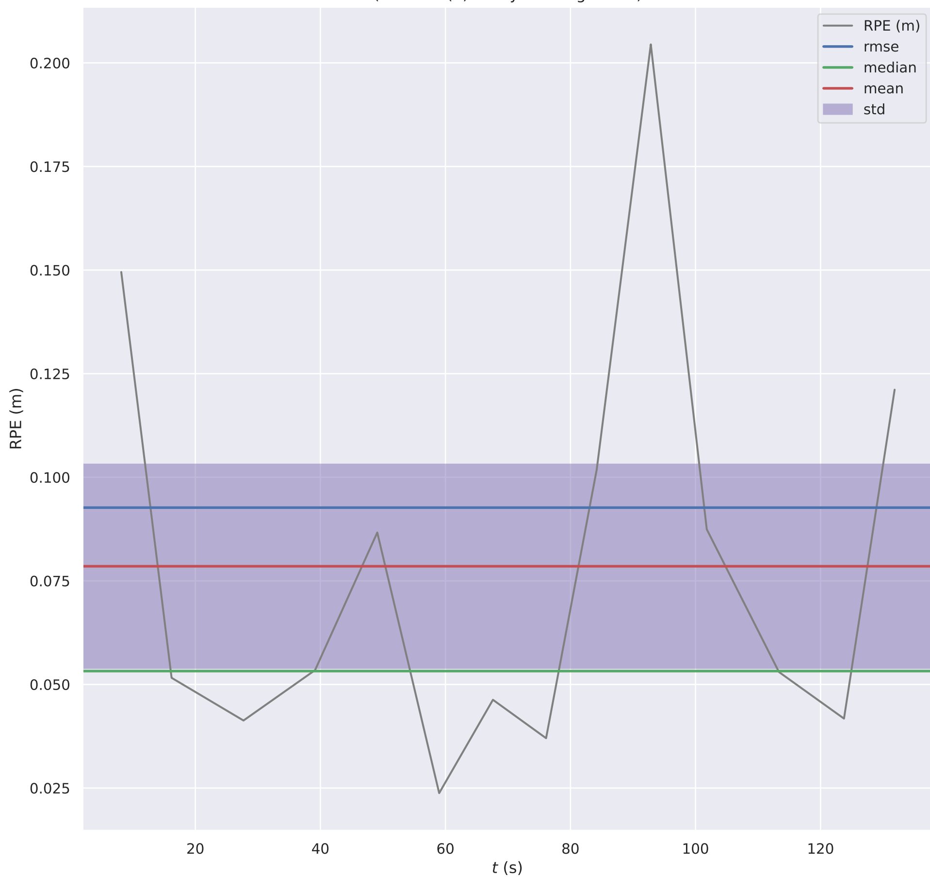
RPE w.r.t. translation part (m) for \delta = 20 (frames) using consecutive pairs (with Sim(3) Umeyama alignment)
