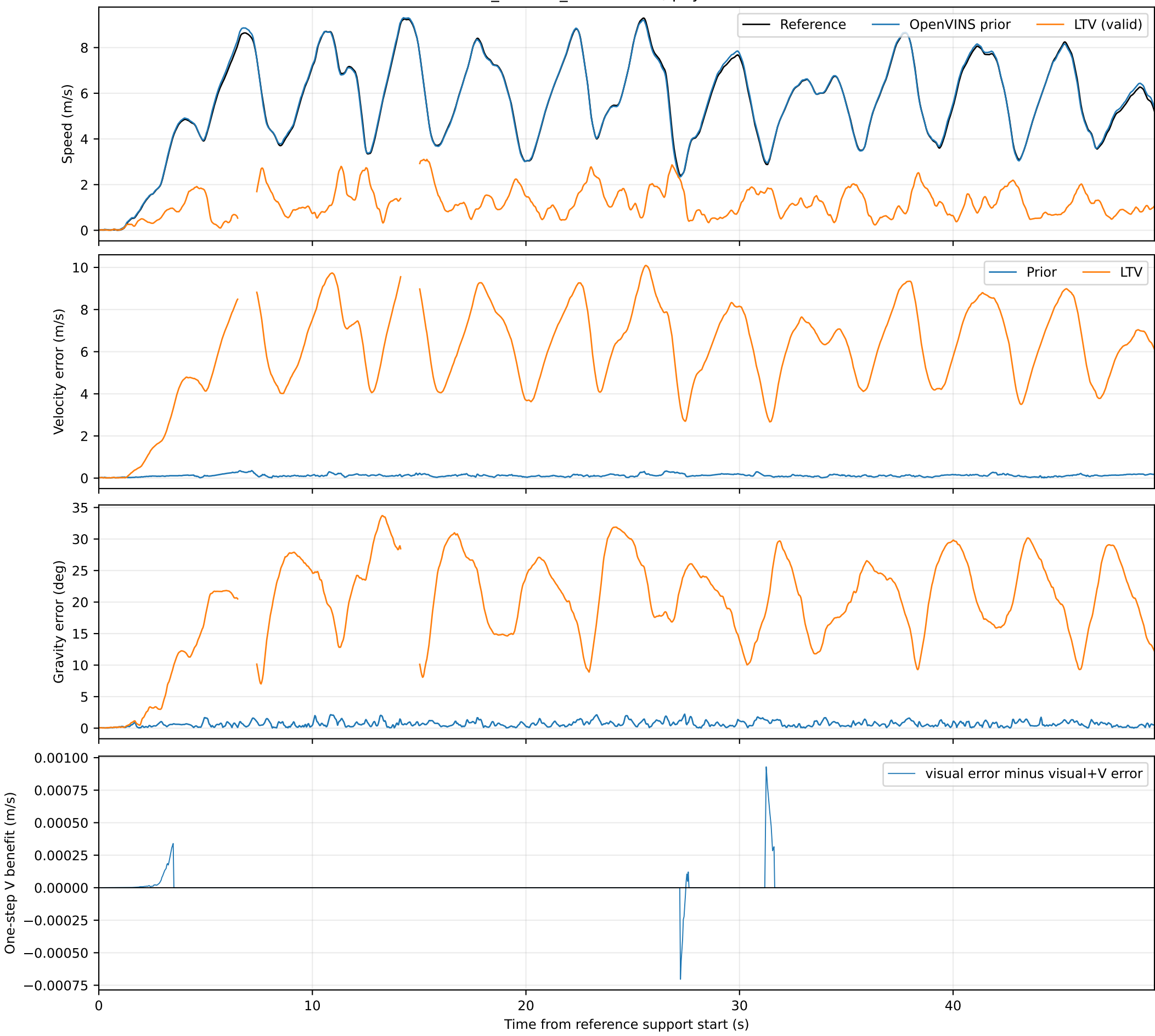
indoor_forward_3 — Passive, physical IMU time
