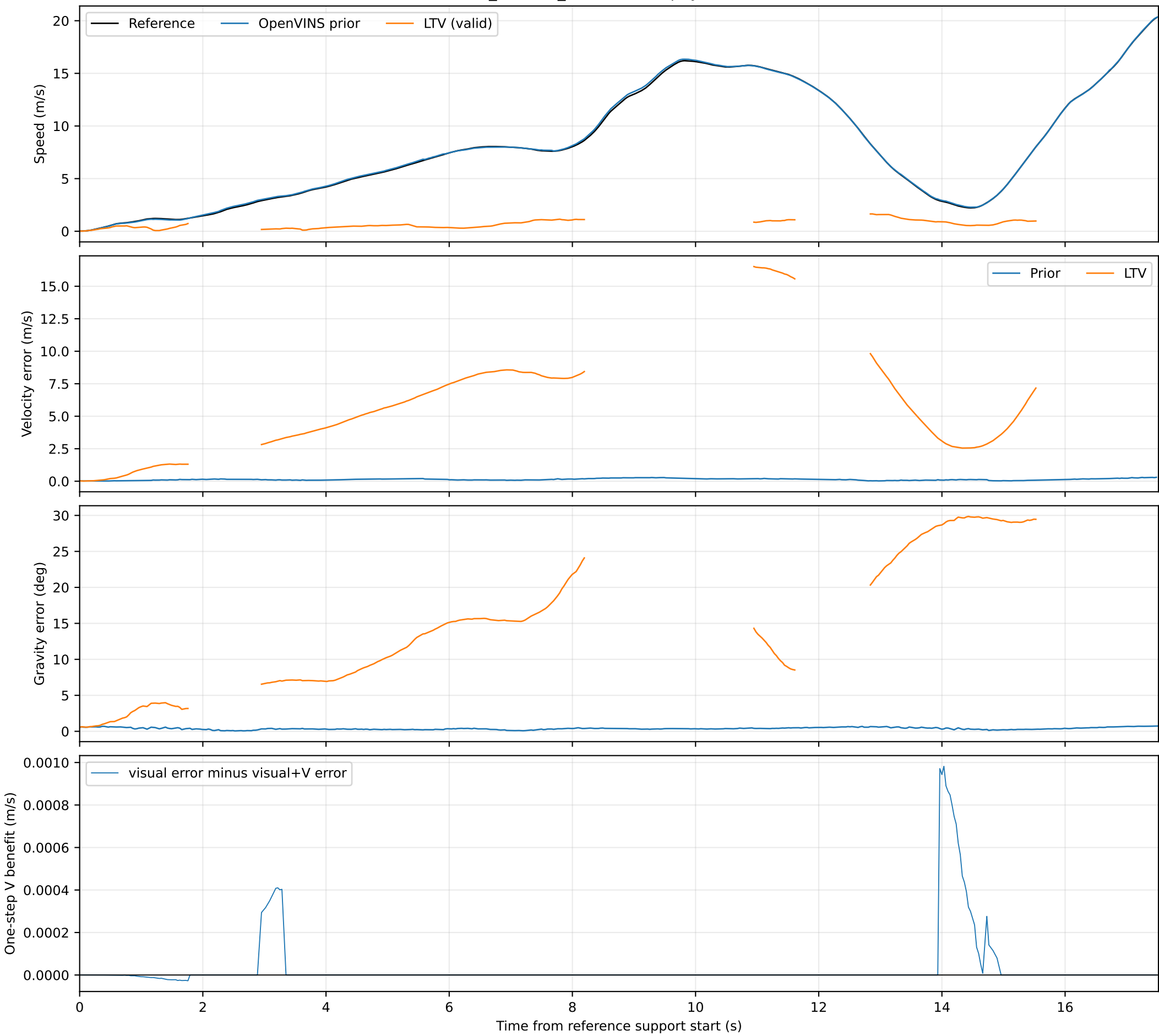
outdoor_forward_5 — Passive, physical IMU time
