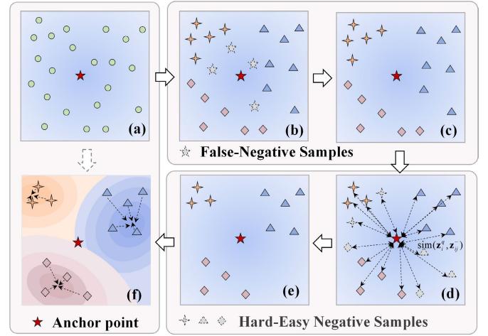
Fig. 3. Details of the negative samples' mining strategies. (a) RNS in traditional contrastive learning, where samples are unlabeled and randomly distributed. (b) Pseudolabels generated by the classifier are assigned to each sample, where false-negative samples are identified. (c) False-negative samples are eliminated based on FNSM strategy. (d) The spatial-spectral joint similarity between the anchor and negative samples is calculated to represent the hardness level of the negative samples. (e) HENSM is conducted by controlling the hardness level of the negative samples. (f) Contrastive learning adjusts the representation by pulling similar samples closer and pushing dissimilar samples farther apart. In this framework, to facilitate the comparisons, (a) and (f) illustrate traditional RNS in contrastive learning, (b) and (c) demonstrate the FNSM strategy, while (d) and (e) represent the HENSM strategy.
