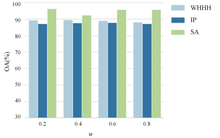
Fig. 7. Classification performance for the IP, WHHH, and SA datasets under different weights.
