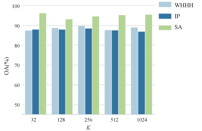
Fig. 8. Classification performance for the IP, WHHH, and SA datasets under different number of negative samples.
