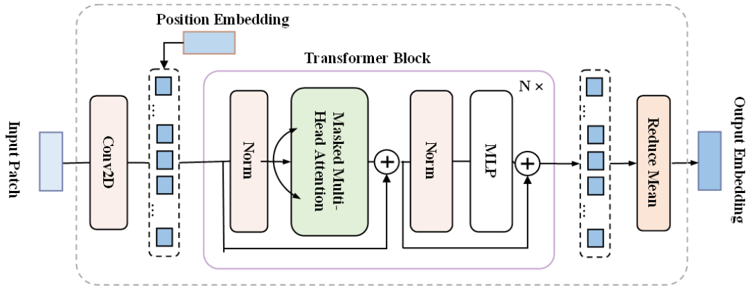
Fig. 2. Detailed structure of the encoder block.
