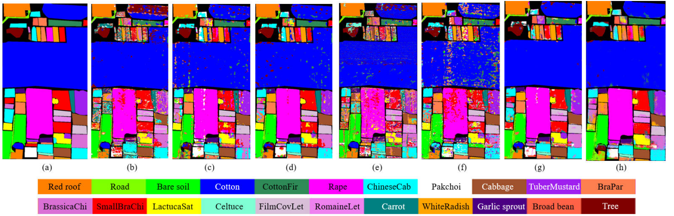
Fig. 11. Visual classification results of WHU-Hi-HongHu from compared methods. (a) Ground truth. (b) HiT. (c) SSFTT. (d) CASST. (e) SC-EADNet. (f) S3Net. (g) C-SS-MTr. (h) Ours.
