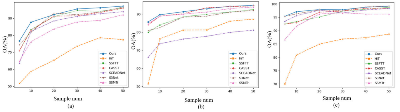
Fig. 9. Overall classification accuracy of various algorithms under different training sample sizes. (a) IP. (b) WHHH. (c) SA.
