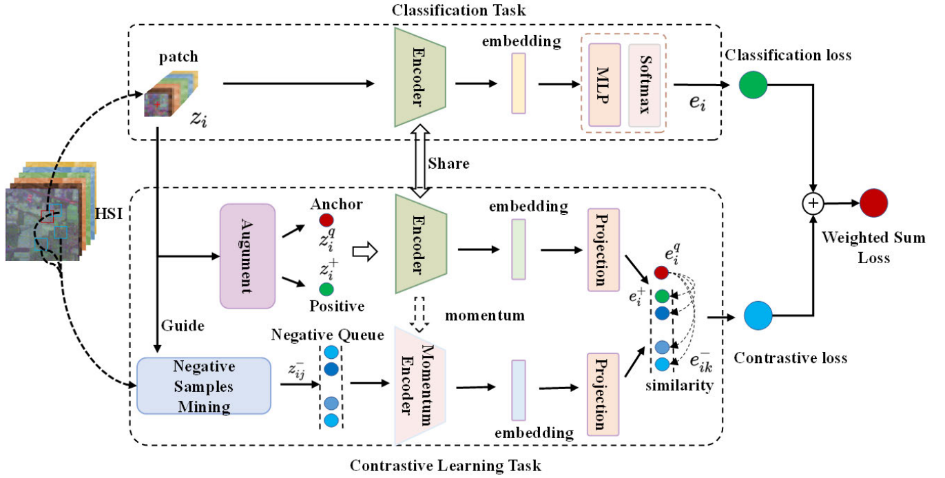
Fig. 1. Framework of our proposed method, which consists of two training tasks: classification task and contrastive learning task.
