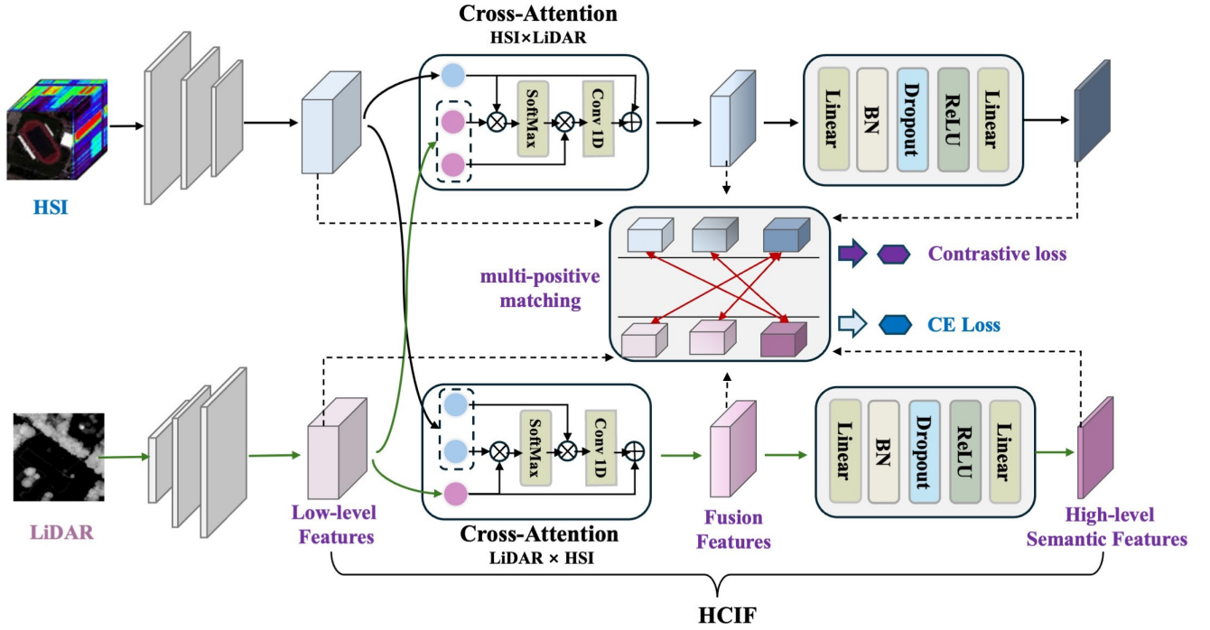
Fig. 1. Framework of the proposed mPMCL method.
