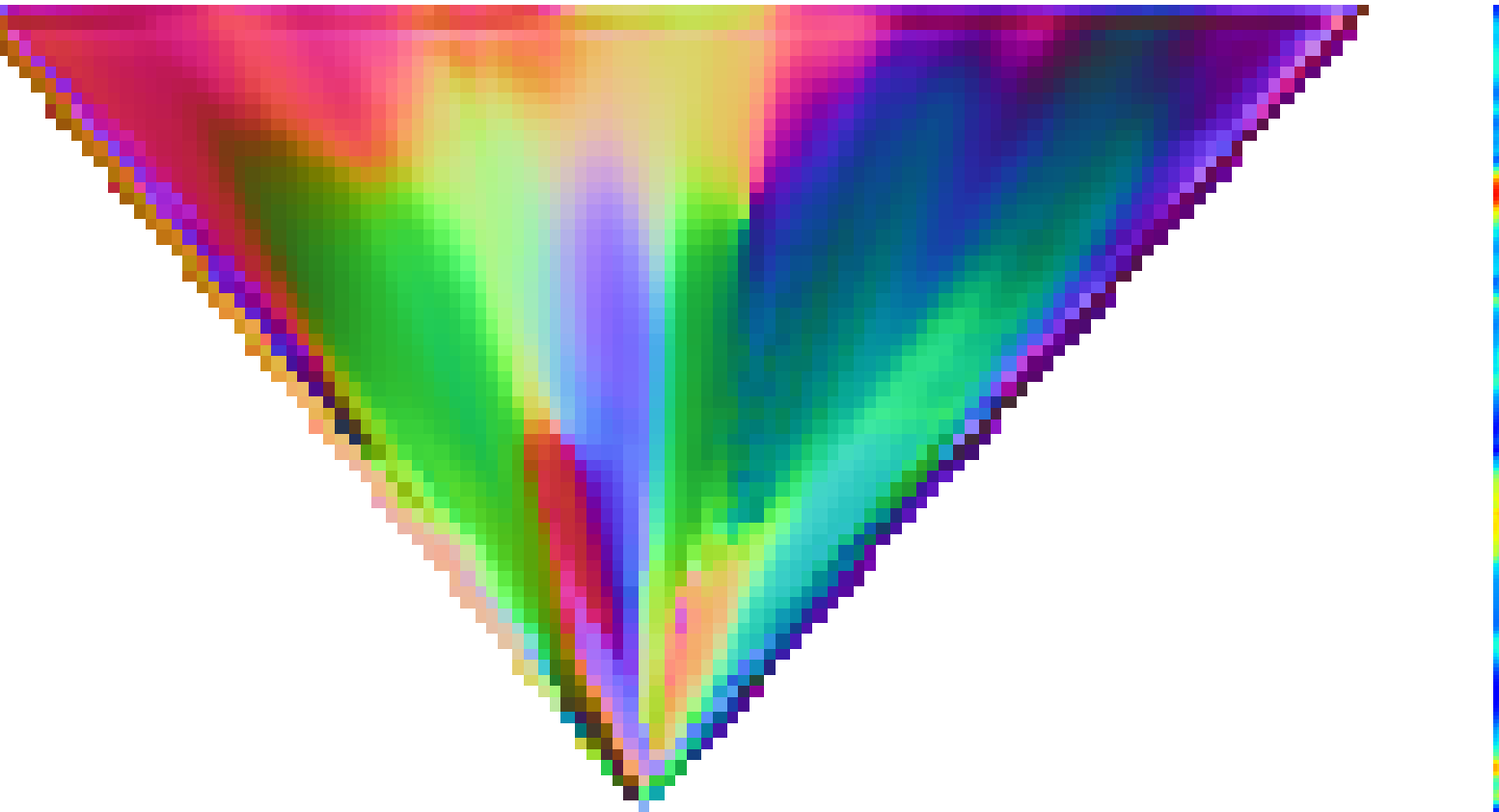
BEV features
