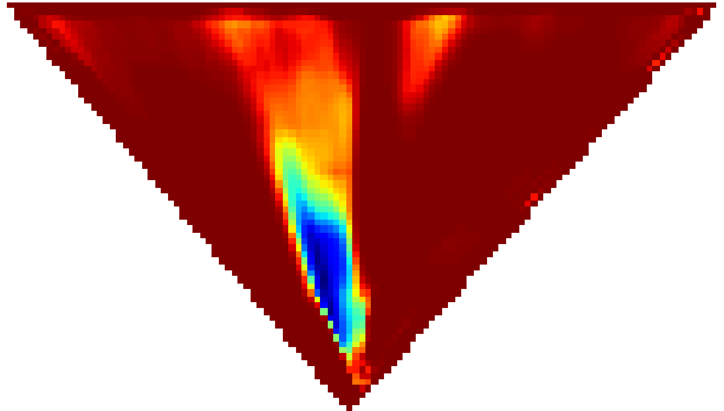
BEV confidence
